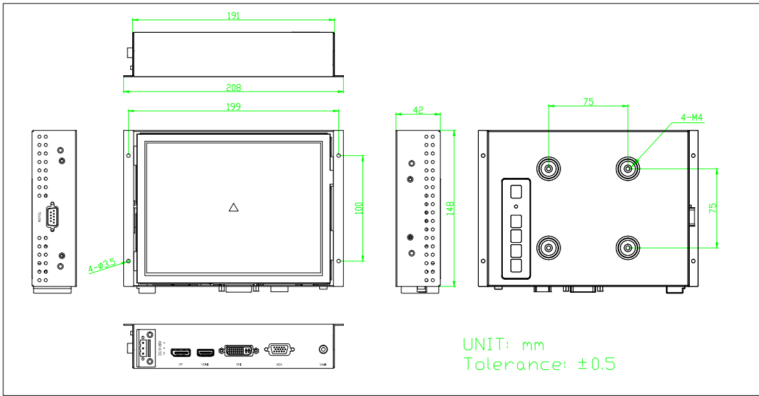
OPD-1086C RS-232
