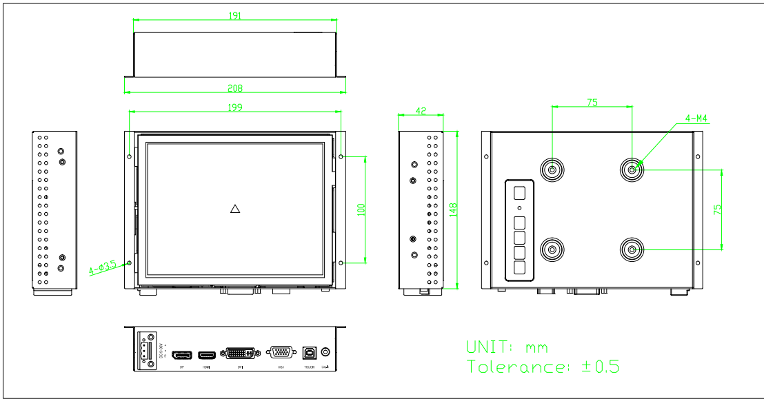
OPD-1086C USB
